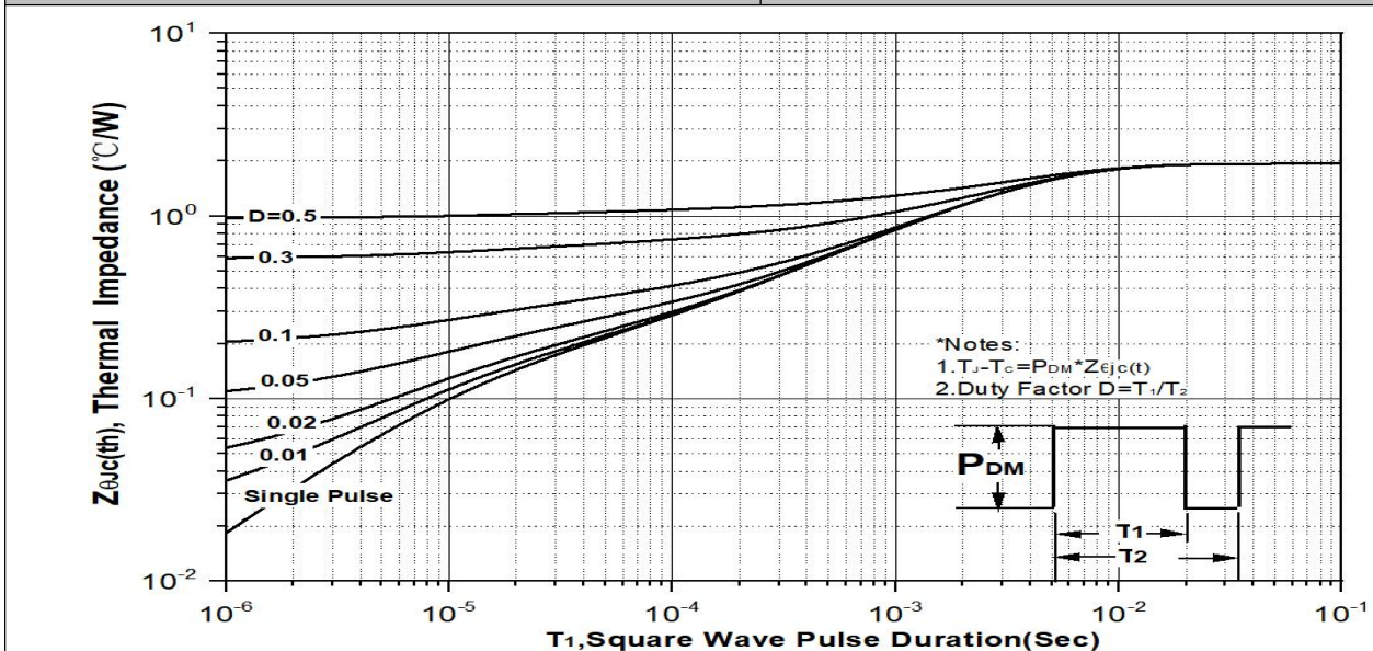
Figure 11. Transient Thermal Impedance
