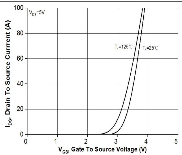
Figure 8. Transfer Characteristics
