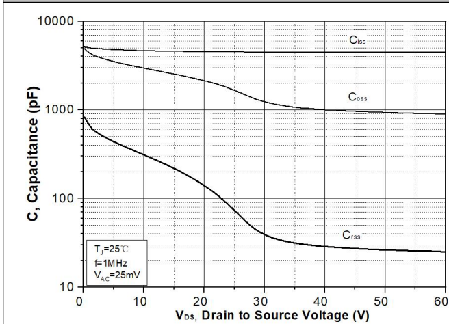
Figure 9. Capacitance
