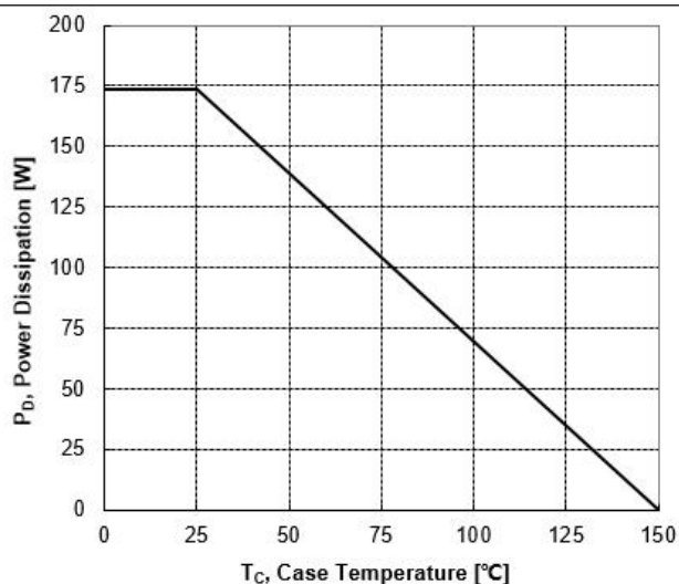
Figure 11. Maximum Power Dissipation vs Case Temperature
