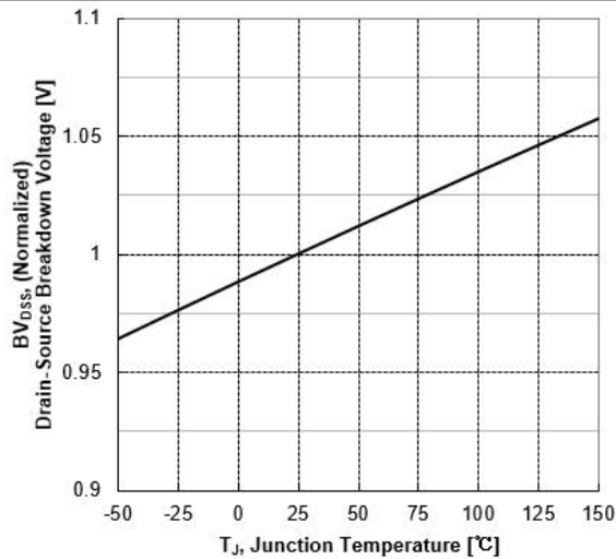
Figure 7. Normalized Breakdown voltage vs Junction Temperature
