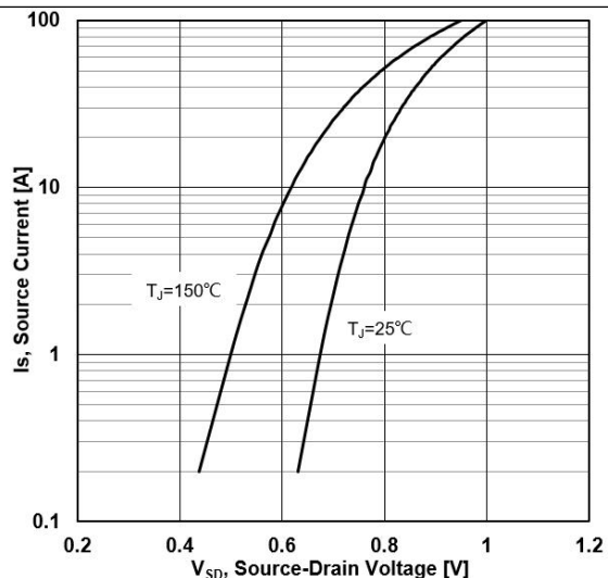
Figure 6. Body Diode Characteristics
