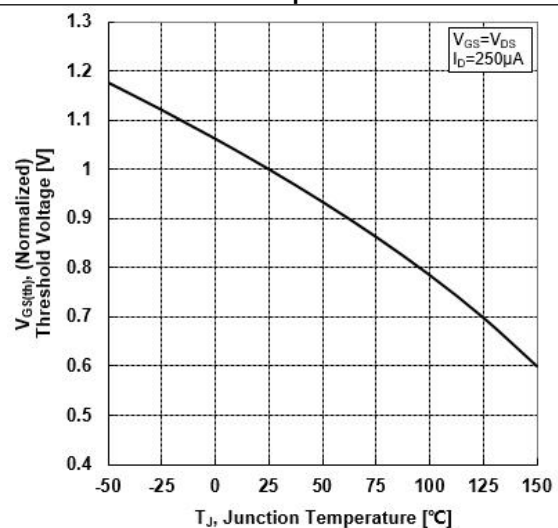
Figure 12. Normalized Threshold Voltage vs Junction Temperature
