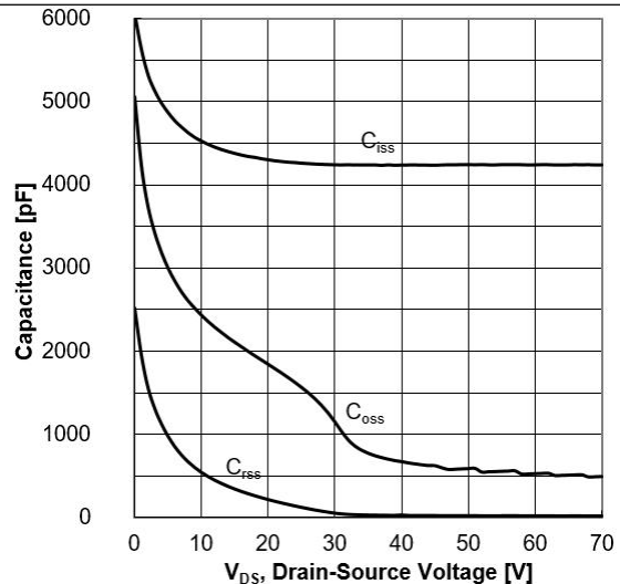
Figure 4. Typical Capacitance
