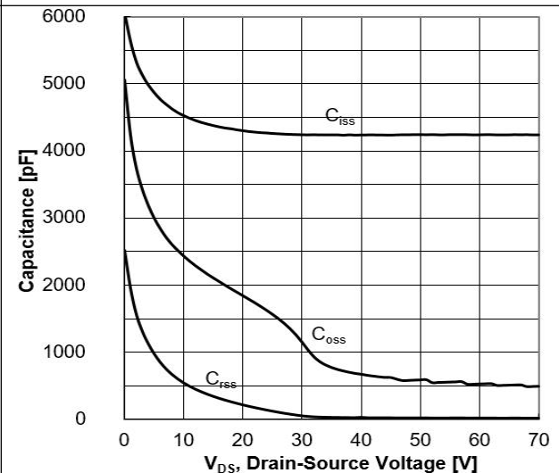
Figure 4. Typical Capacitance
