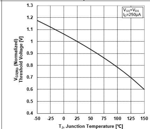
Figure 12. Normalized Threshold Voltage vs Junction Temperature
