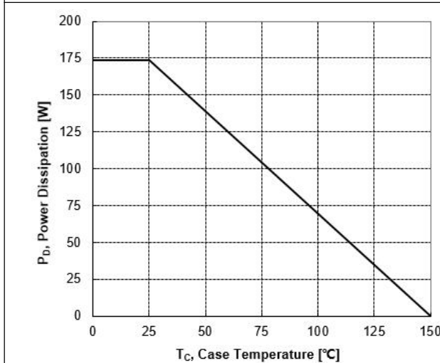
Figure 11. Maximum Power Dissipation vs Case Temperature
