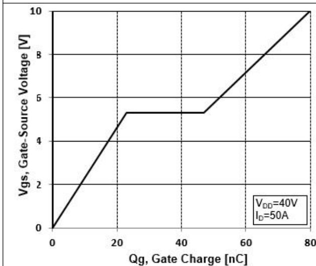
Figure 3. Typical Gate Charge
