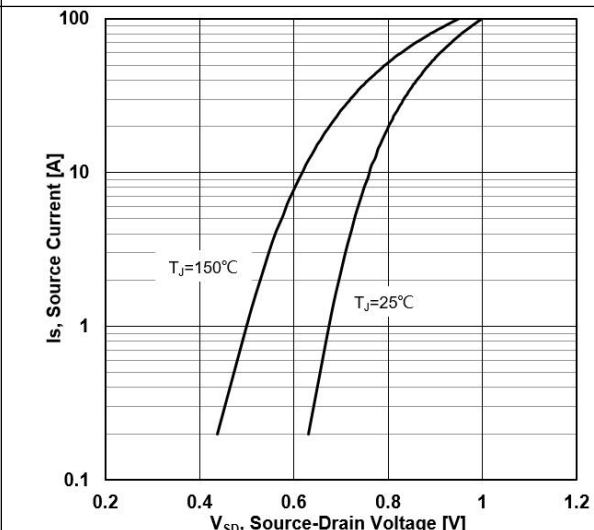
Figure 6. Body Diode Characteristics
