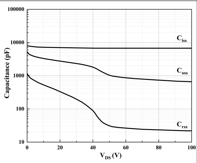
Figure 4. Typical Capacitance
