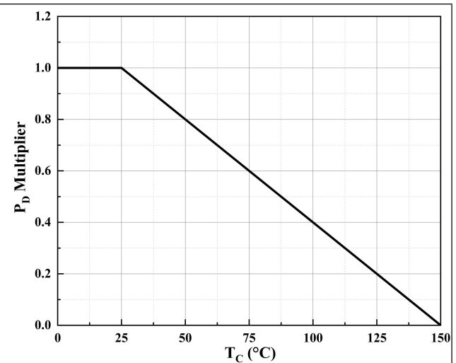
Figure 8. Maximum Power Dissipation Multiplier vs. Case Temperature
