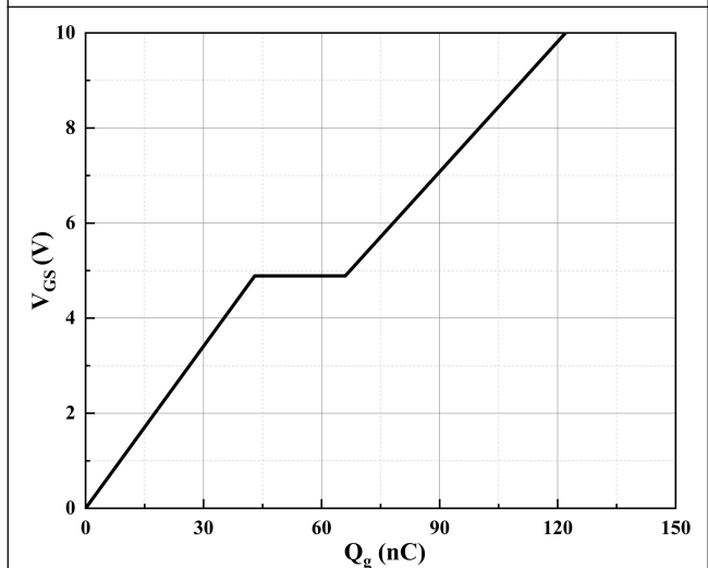
Figure 3. Typical Gate Charge
