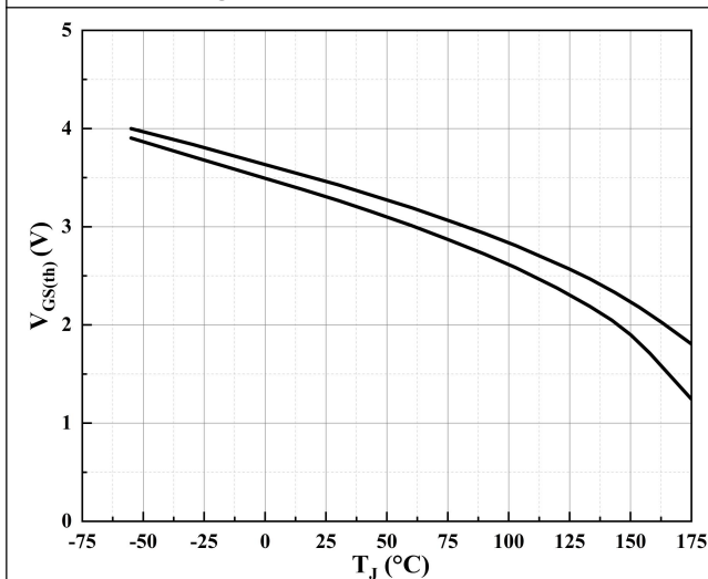
Figure 11. Gate Threshold Voltage vs. Junction Temperature
