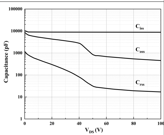
Figure 4. Typical Capacitance
