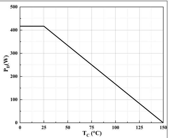
Figure 8. Maximum Power vs. Case Temperature
