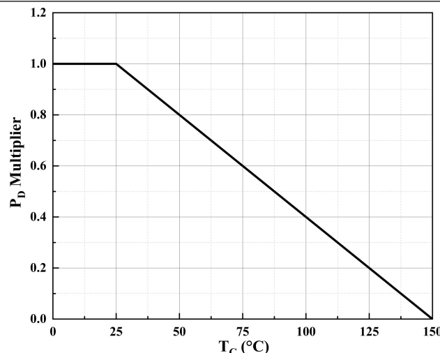
Figure 10. Maximum Power Dissipation Multiplier vs. Case Temperature
