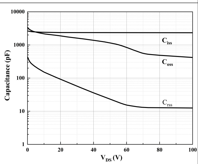
Figure 6. Typical Capacitance
