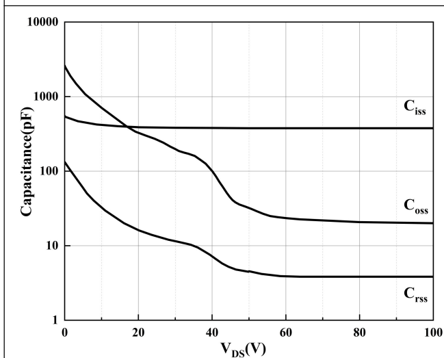
Figure 5. Typical Capacitance
