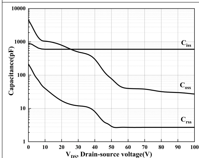
Figure 5. Typical Capacitance
