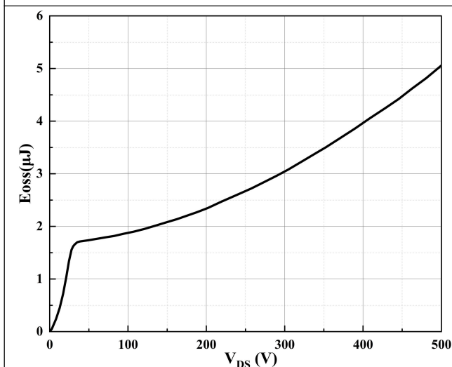
Figure 5. Typical Coss Stored Energy
