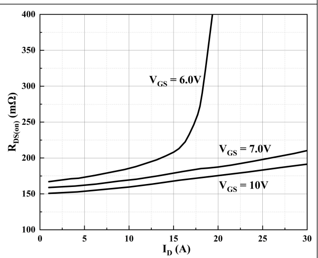
Figure 6. Static Drain-Source On-Resistance vs. Drain Current
