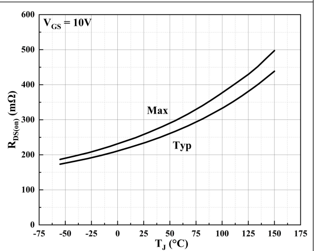
Figure 10. Static Drain-Source On-Resistance vs. Junction Temperature
