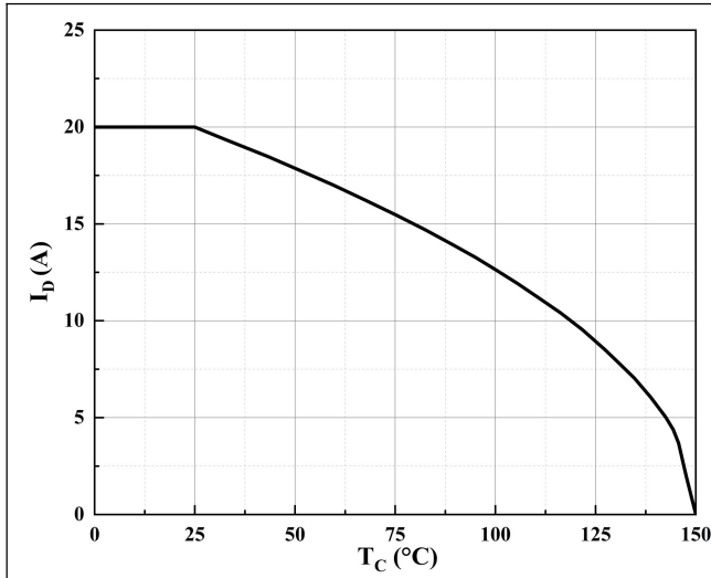
Figure 7. Continuous Drain Current vs. Case Temperature
