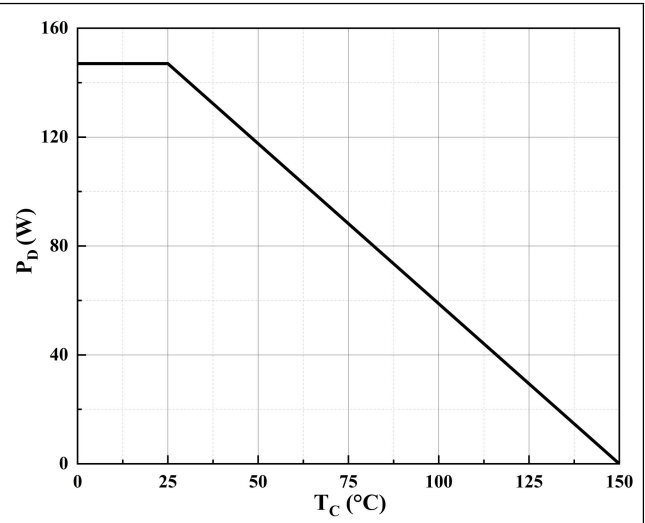
Figure 8. Power Dissipation vs. Case Temperature
