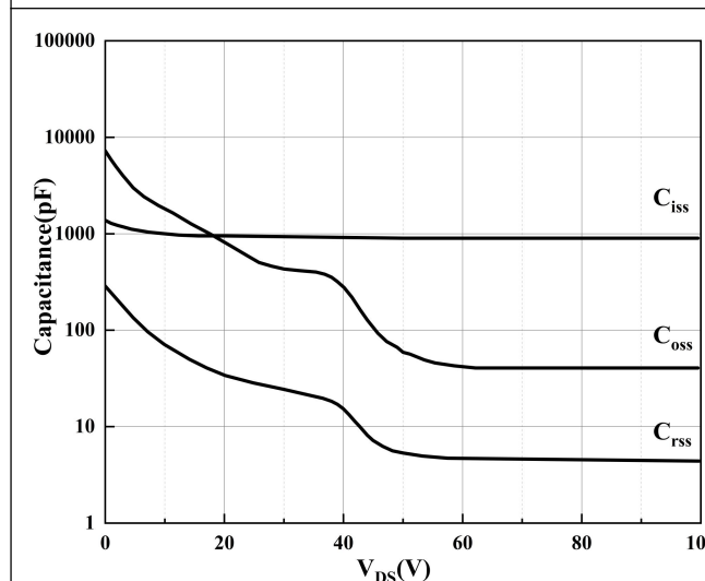
Figure 5. Typical Capacitance
