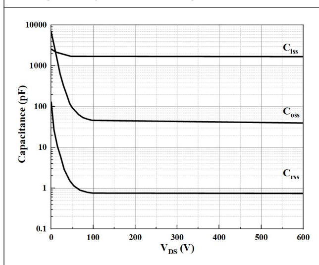
Figure 5. Typical Capacitance
