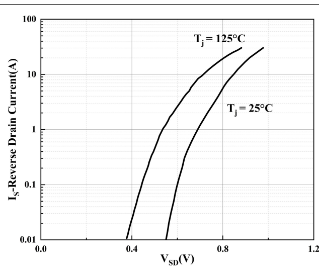
Figure 4. Forward Characteristics of Reverse Diode
