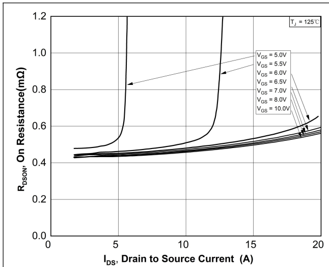
Figure 7. Typical drain-source on-state resistance
