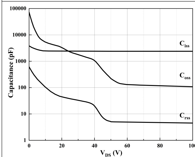
Figure 5. Typical Capacitance
