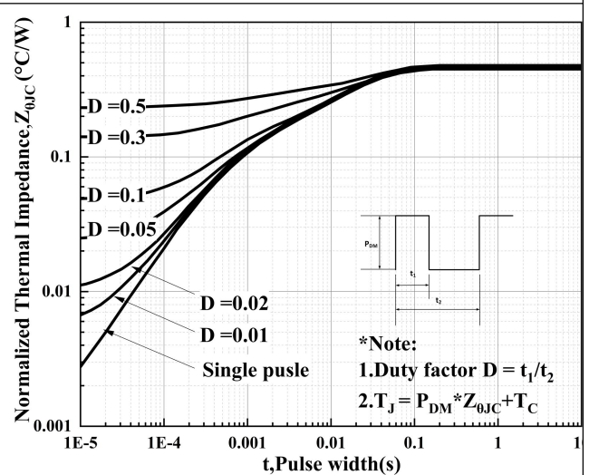
Figure 10. Maximum transient thermal impedance
