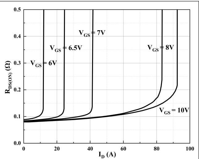
Figure 8. Typical Drain-source On-state Resistance
