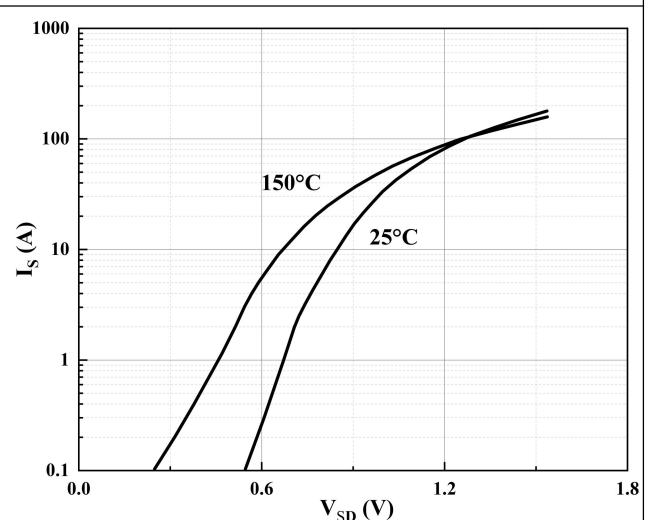
Figure 12. Forward characteristics of reverse diode
