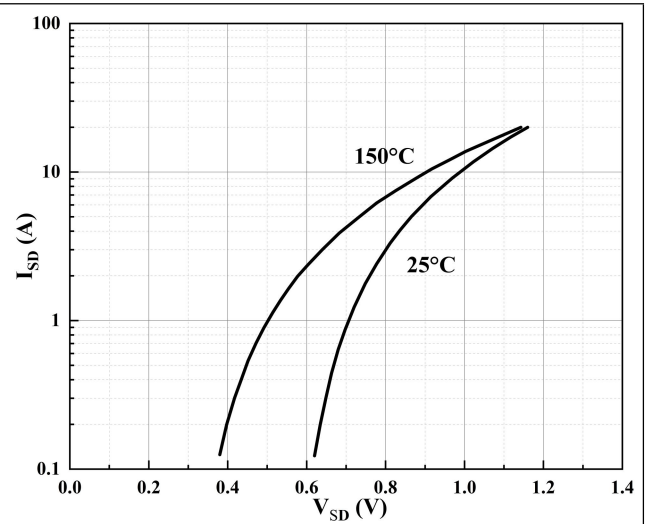
Figure 8. Body-Diode Characteristics
