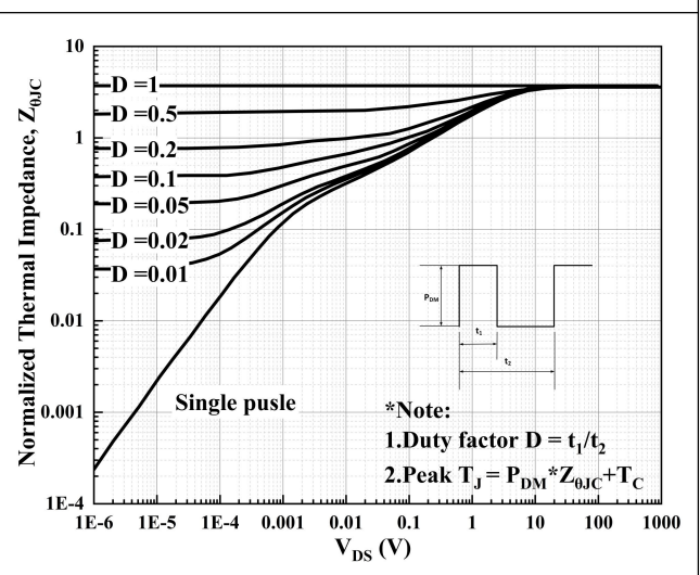
Figure 12. Maximum Transient Thermal Impedance
