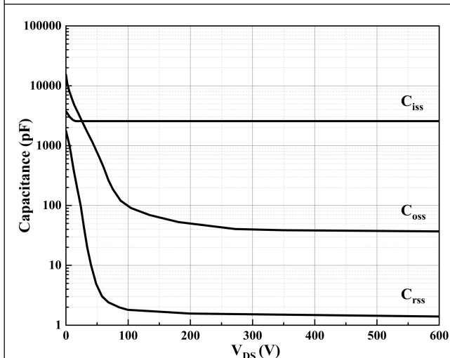
Figure 5. Typical Capacitance
