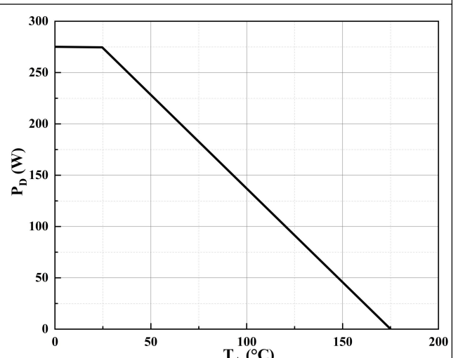
Figure 6. Typical Power Dissipation
