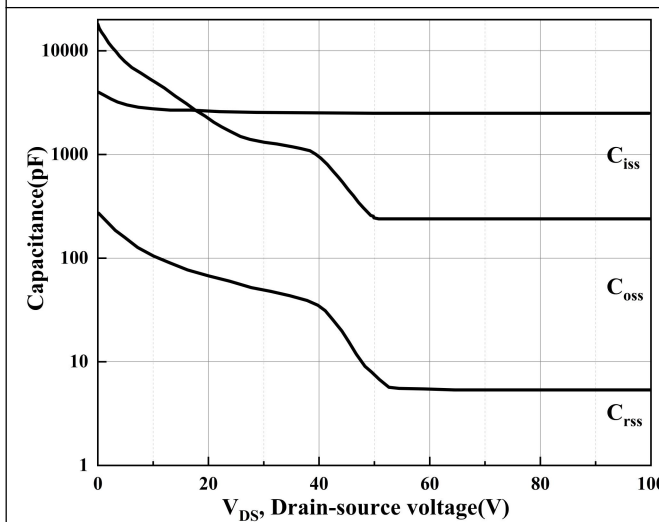
Figure 5. Typical Capacitance
