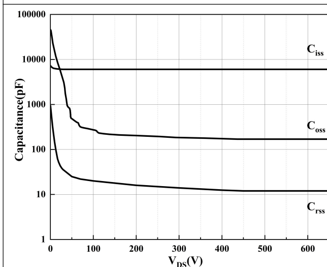
Figure 5. Typical Capacitance
