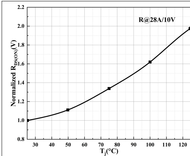
Figure 7. Typical On-Resistance vs Junction Temperature
