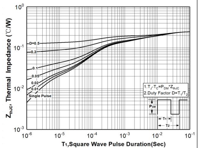
Figure 12. Typ. Max. transient thermal impedance
