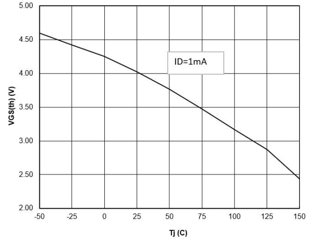
Figure 8. Typ. Threshold voltage
