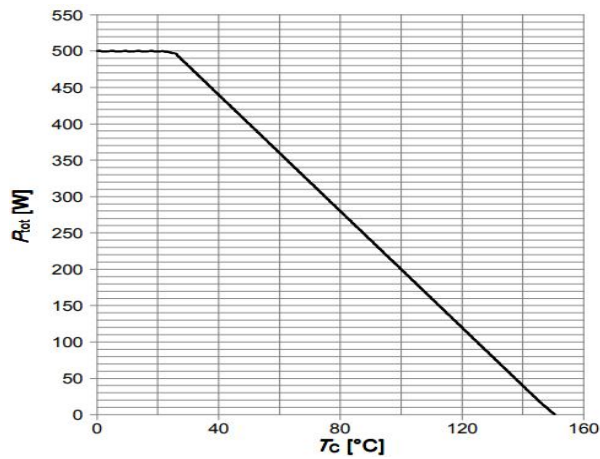
Figure 9. Typ. Power Dissipation
