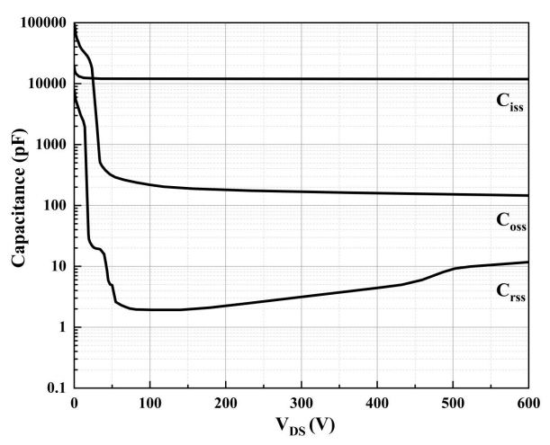
Figure 4. Typical Capacitance
