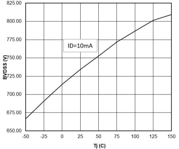
Figure 6. Drain-source Breakdown Voltage
