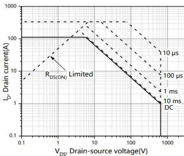
Figure 11. Typ. Maximum Safe Operating Area
