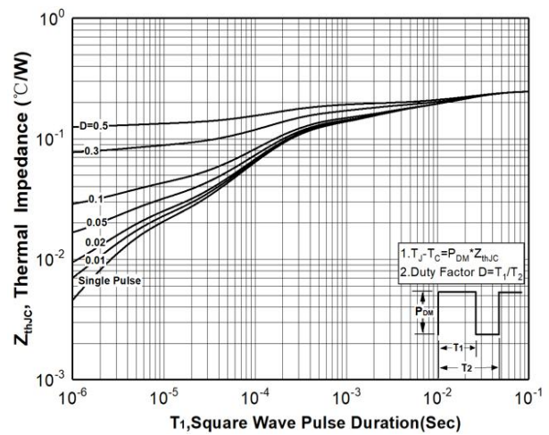
Figure 12. Typ. Max. transient thermal impedance
