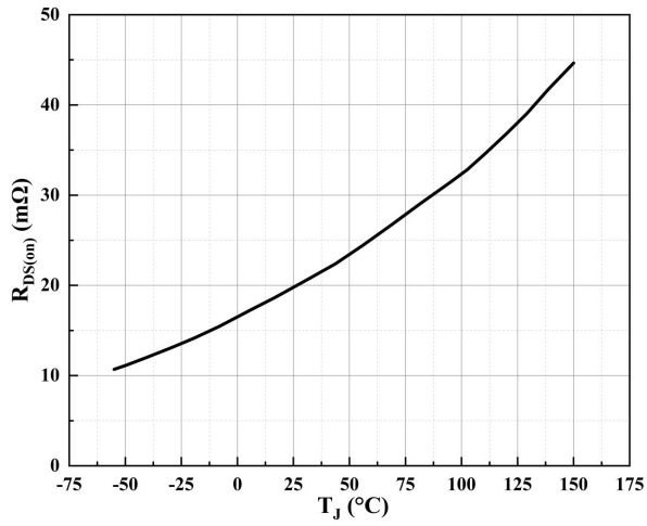
Figure 7. Typical On-Resistance vs Junction Temperature
