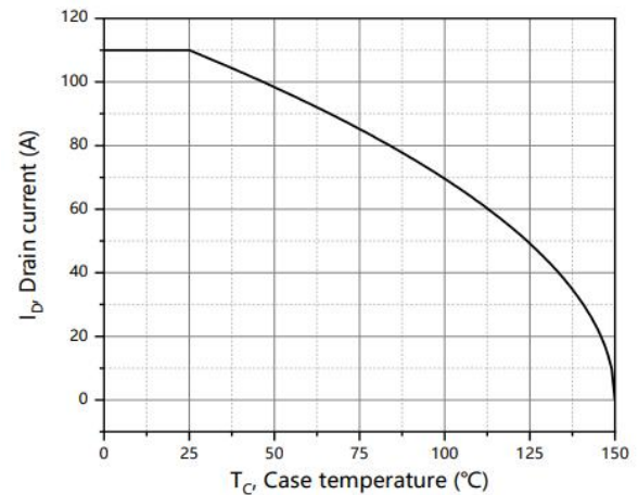
Figure 10. Typ. Drain Current De-rating
