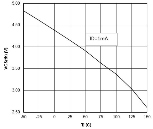
Figure 8. Typ. Threshold voltage
