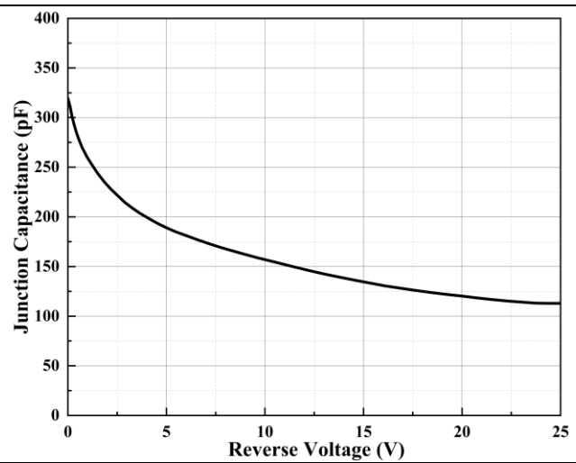
Figure 2. Junction Capacitance vs. Reverse Voltage
