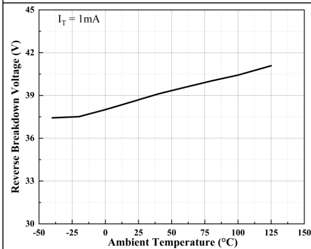
Figure 3. Reverse Breakdown Voltage vs. Ambient Temperature
