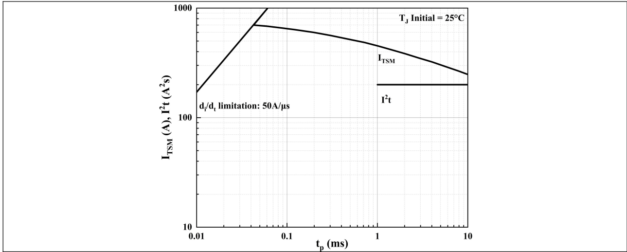
Figure 7. Non-Repetitive Surge Peak On-State Current for a Sinusoidal Pulse with Width t_p < 10 ms and Corresponding Value of I^2t ( d_i/d_t < 50 A/μs)
