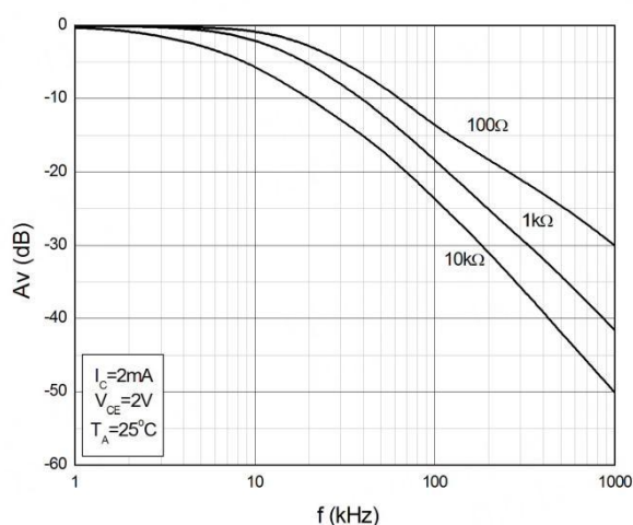
Fig.11 Frequency Responses
