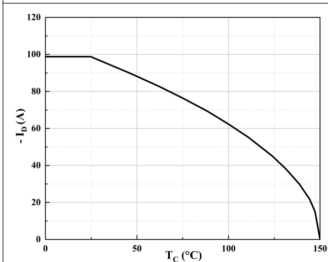
Figure 5. Maximum Continuous Drain Current vs Case Temperature
