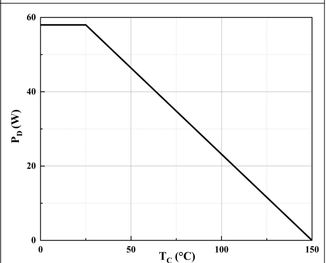
Figure 6. Power Dissipation
