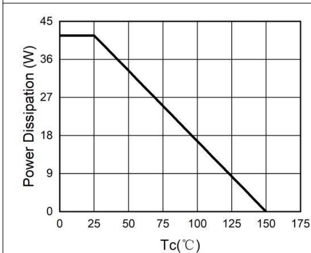
Figure 5. Power Dissipation
