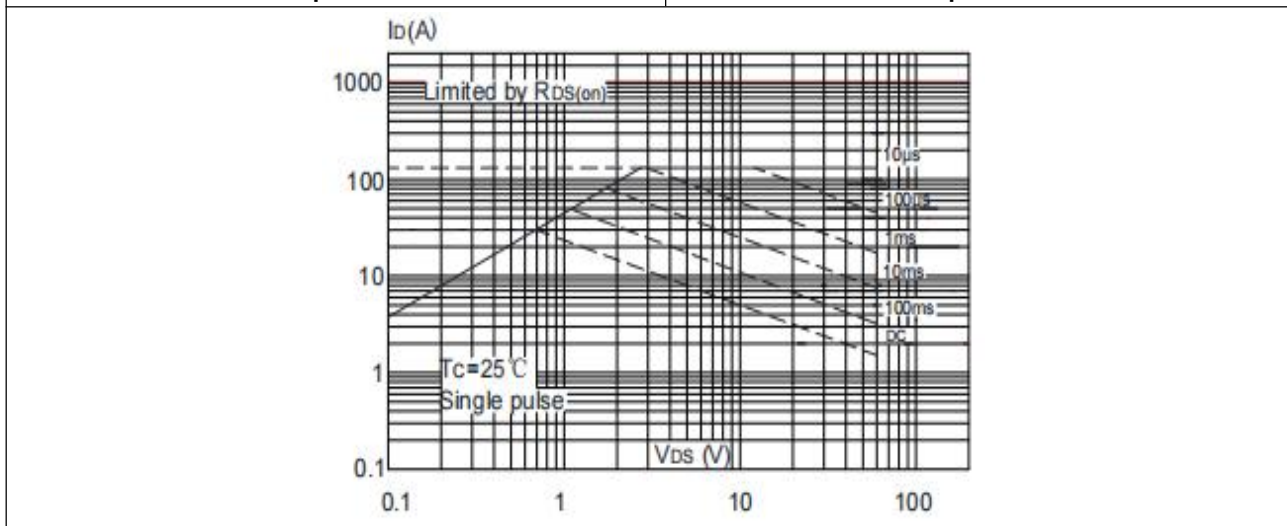
Figure 11. Maximum Safe Operating Area
